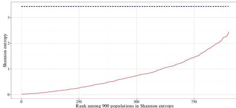
FIG 1. The empirical Shannon entropy in the microbial distribution across 900 samples of the vaginal microbiome (Ravel et al. [59]), which are ranked according to the level of diversity. The dashed blue line shows the Shannon entropy of the Uniform distribution for the same number of species.
